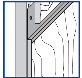
J. Z-Flashing – Prevents leakage where two pieces of siding meet.
