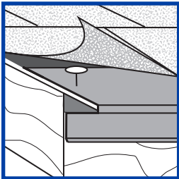
A. Drip Edge – Diverts water away from house along entire eave.
