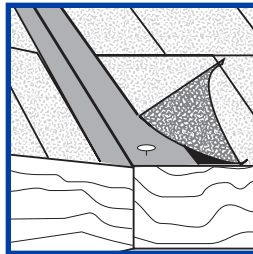
H. Rolled Flashing – Prevents water penetration where two roof faces meet.
