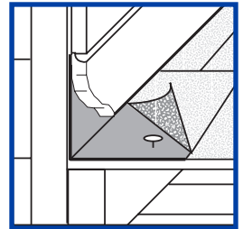
E. Angle Flashing – Prevents water infiltration at a wall. Diverts water away from house.
