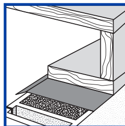
L. Termite Shield – Prevents termites from getting access to sills and wooden structure.
