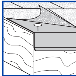
B. Eave Edge – Diverts water away from house along entire eave.
