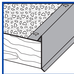
K. Gravel Stop – Prevents gravel from washing off a gravel roof. Apply across entire eave.
