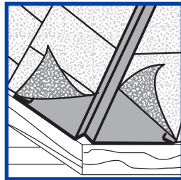
G. Preformed Valley – Prevents water penetration at valley.
