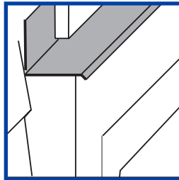
C. Drip Cap – Diverts water away from windows and doors.
