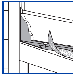
D. Shingle Endwall Flashing – Prevents water infiltration at a wall. Diverts water away from house.
